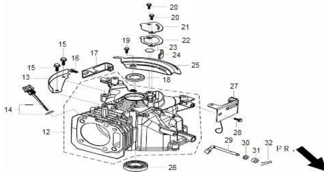
FIG.2 CRANKCASE/GOVERNOR GEAR ASSEMBLY
